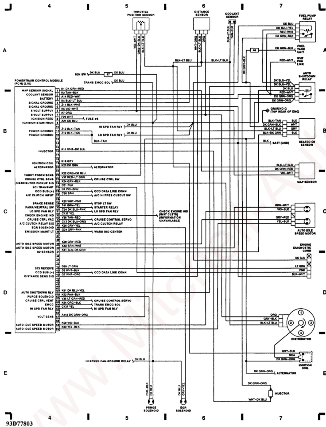
Fig. 2: Electronic Control Module (2.5L) (Grids 4-7)
