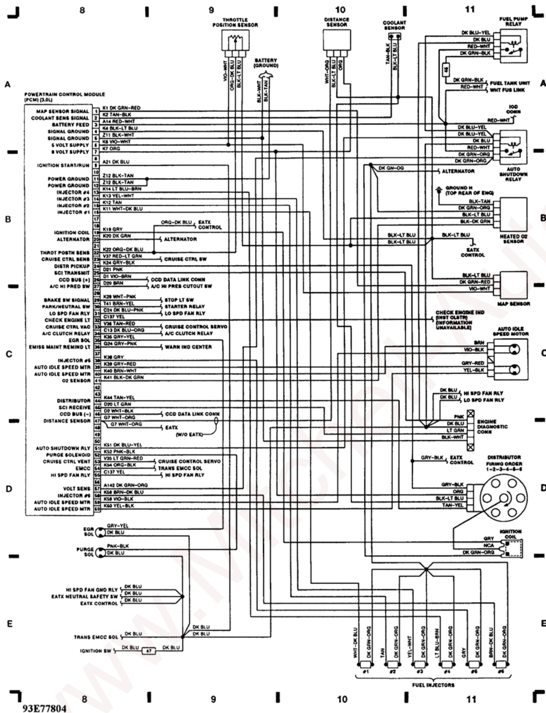
Fig. 3: Electronic Control Module (3.0L) (Grids 8-11)
