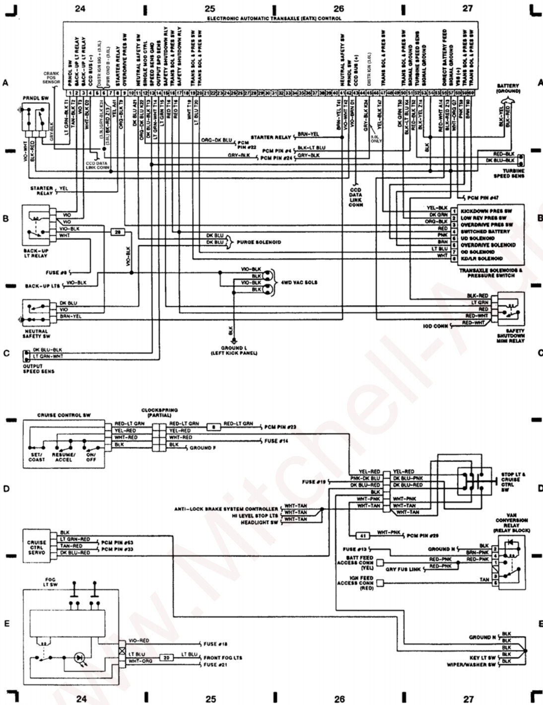
Fig. 7: EATX Control System & Cruise Control (Grids 24-27)
