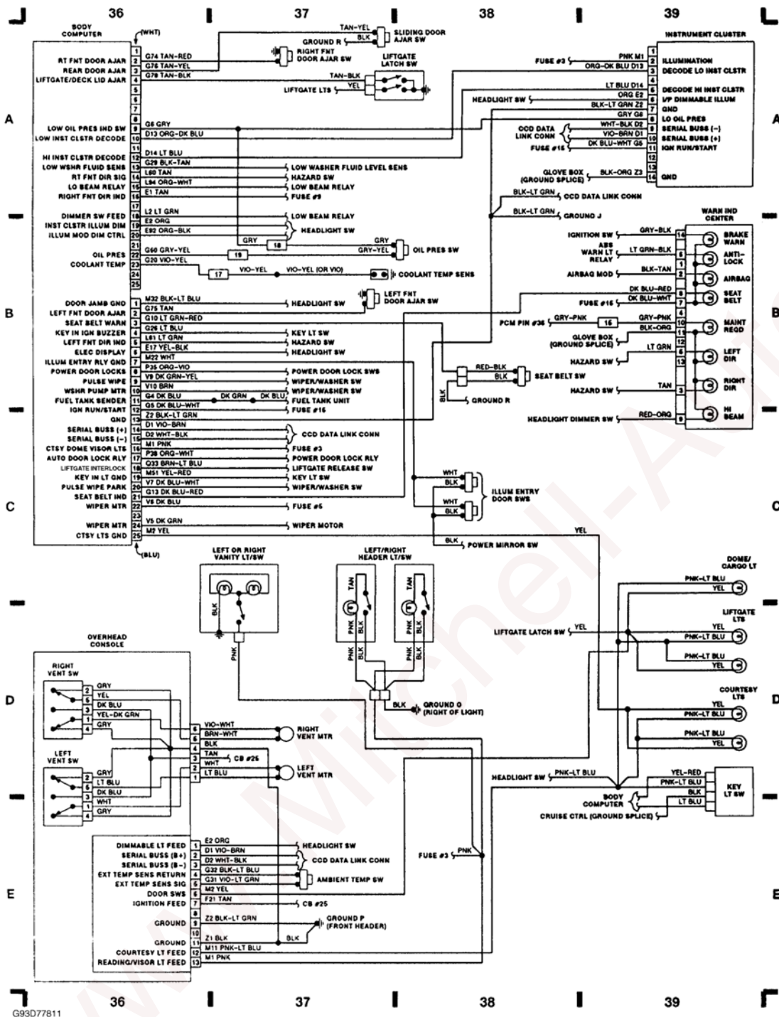
Fig. 10: Body Computer/Overhead Console/Inst. Clstr. (Grids 36-39)
