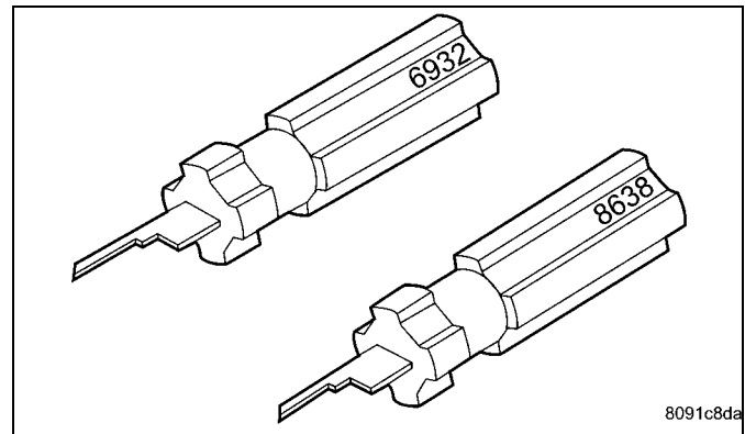
TERMINAL REMOVING TOOLS 6932 AND 8638
