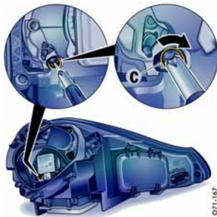
Xenon headlight
