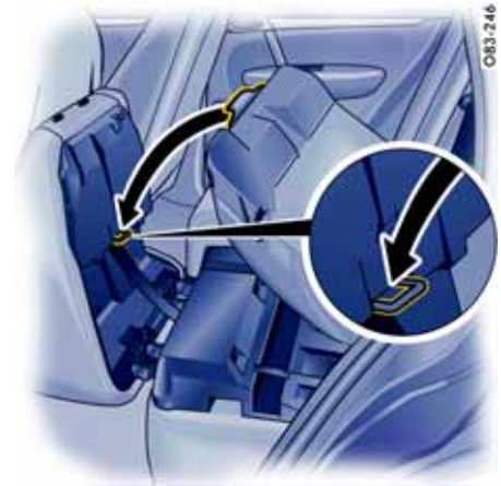
Rear seat assembly for sport seats
