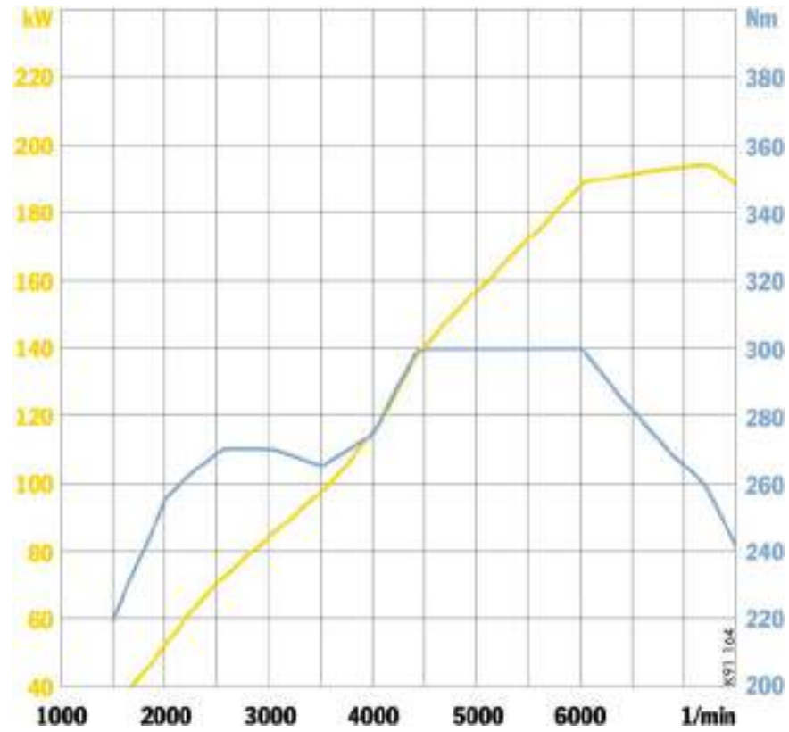
Engine diagram at full power, Cayman
