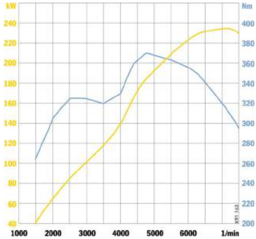
Engine diagram at full power, Cayman S
