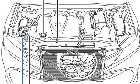
Windshield washer fluid tank Engine coolant reservoir
