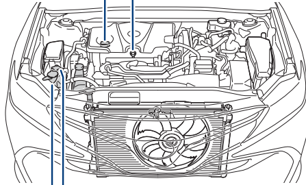
Windshield washer fluid tank Engine coolant reservoir
