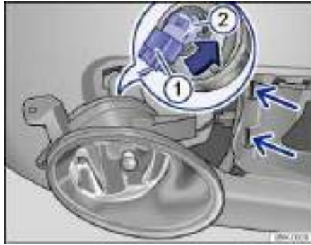
Fig. 194 Replacing a light bulb in the fog light.
