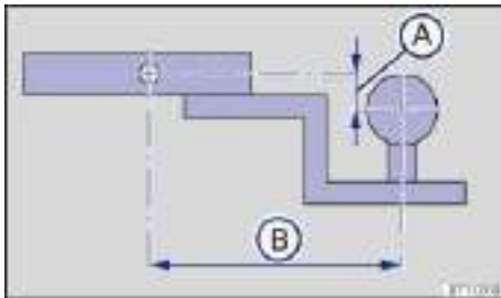
Fig. 101 Dimensions of the ball mount support.
