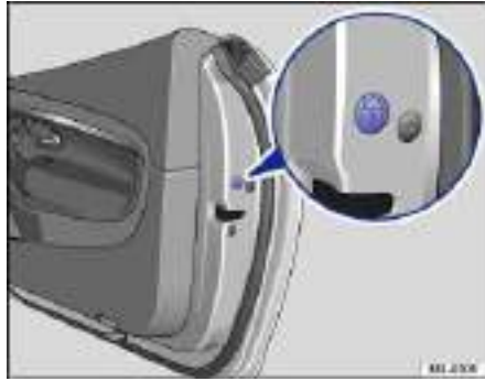
Fig. 165 On the front side of the passenger door: Emergency lock, covered by a rubber seal.
