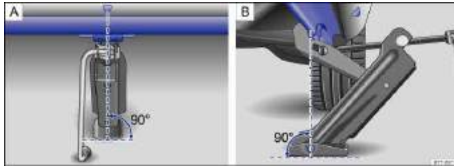
Fig. 186 Jack in position at the left rear lift point.
