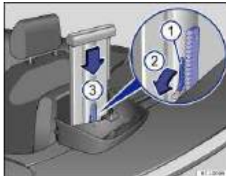
Fig. 174 Deployed rollover protection support behind the rear seat backrest.
