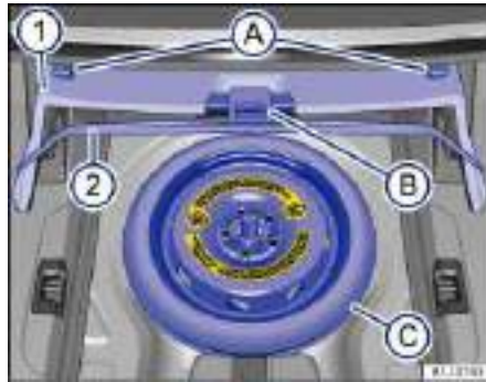
Fig. 106 Compact spare wheel and tire C inside the luggage compartment under the floor covering.
