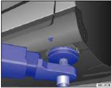
Fig. 161 Front lift point for workshop hoist or floor jack.
