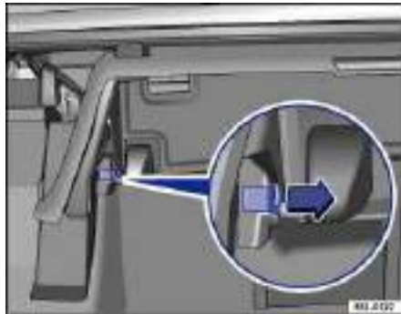
Fig. 98 Removing the inside luggage compartment cover.
