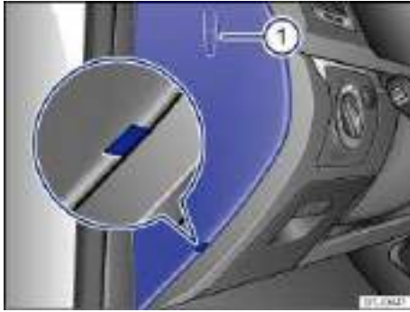
Fig. 188 On the driver side in the instrument panel: Fuse box cover with plastic tweezers 1 on the inside of the cover.
