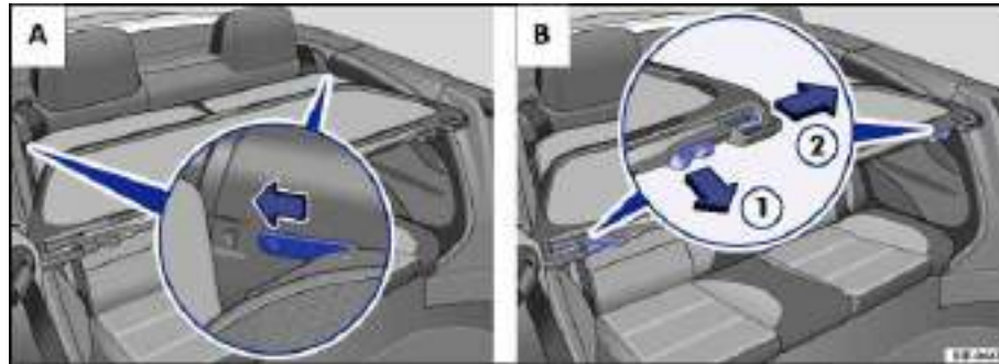
Fig. 33 A. Push tabs (spacers) on wind blocker into slots. B. Align and engage the spring-loaded locking pins.
