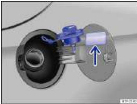
Fig. 149 Fuel cap placed on the open fuel filler flap.
