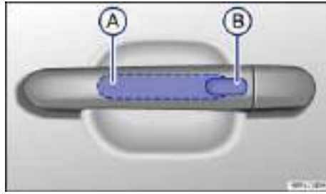
Fig. 26 Keyless Access locking and starting system: Sensor for unlocking A on the inside of the front door handles. Sensor for locking B on the outside of the door handles.
