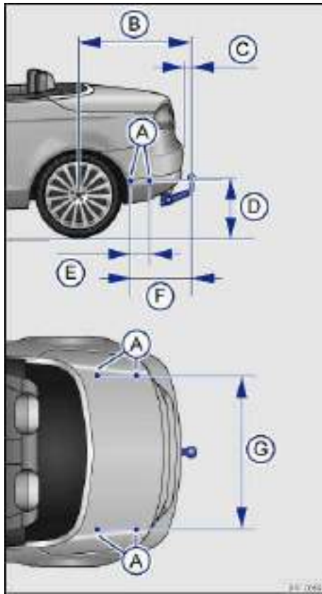
Fig. 102 Dimensions and attachment points for retrofitting a trailer hitch.
