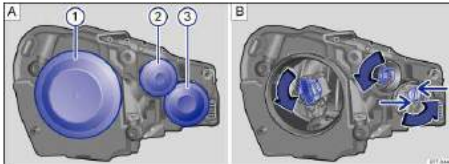
Fig. 192 In the engine compartment: Covers in the left headlight assembly. 1 Low beam, 2 Turn signal indicator, 3 High beam and parking light as well as daytime running light.
