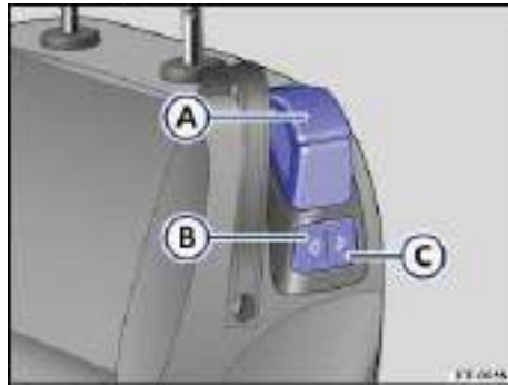
Fig. 45 On the left side of the driver seat: Controls in the backrest for electrical Easy Entry. On the front passenger side, controls are on the right side of the seat backrest.
