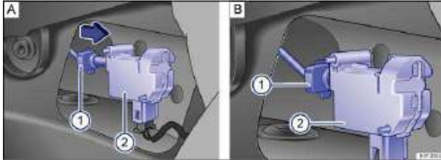
Fig. 170 Right side of luggage compartment: Emergency release of fuel filler flap.
