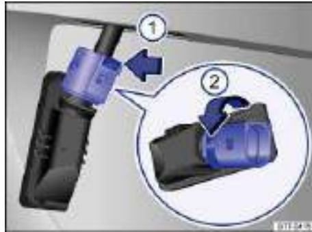
Fig. 196 License plate light: Removing the bulb holder.
