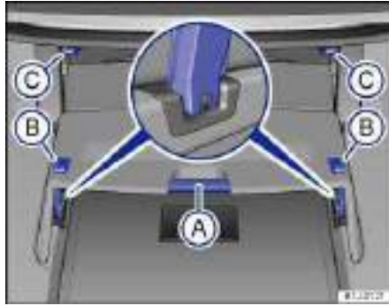
Fig. 97 Lifting up the inside luggage compartment cover.
