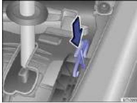
Fig. 176 Releasing the selector lever lock.
