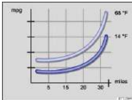
Fig. 135 Fuel consumption in mpg at 2 different outside air temperatures.
