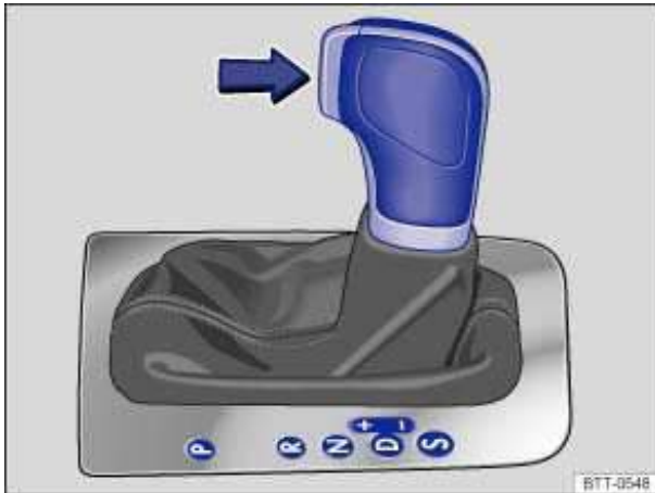
Fig. 133 Side view: Automatic transmission selector lever with shift lever release button (arrow).
