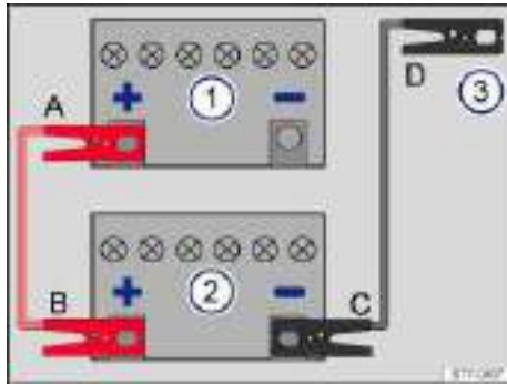
Fig. 210 Diagram for attaching the jumper cables: Dead battery 1 and booster battery 2.
