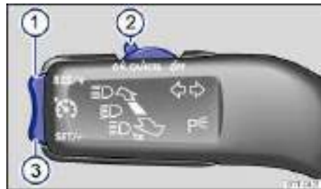
Fig. 149 On the left side of the steering column: Cruise control buttons and switches.
