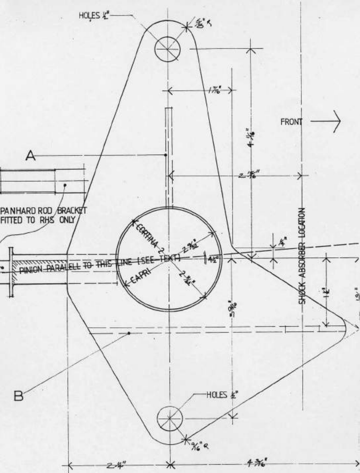
RADIUS ARM BRACKET
