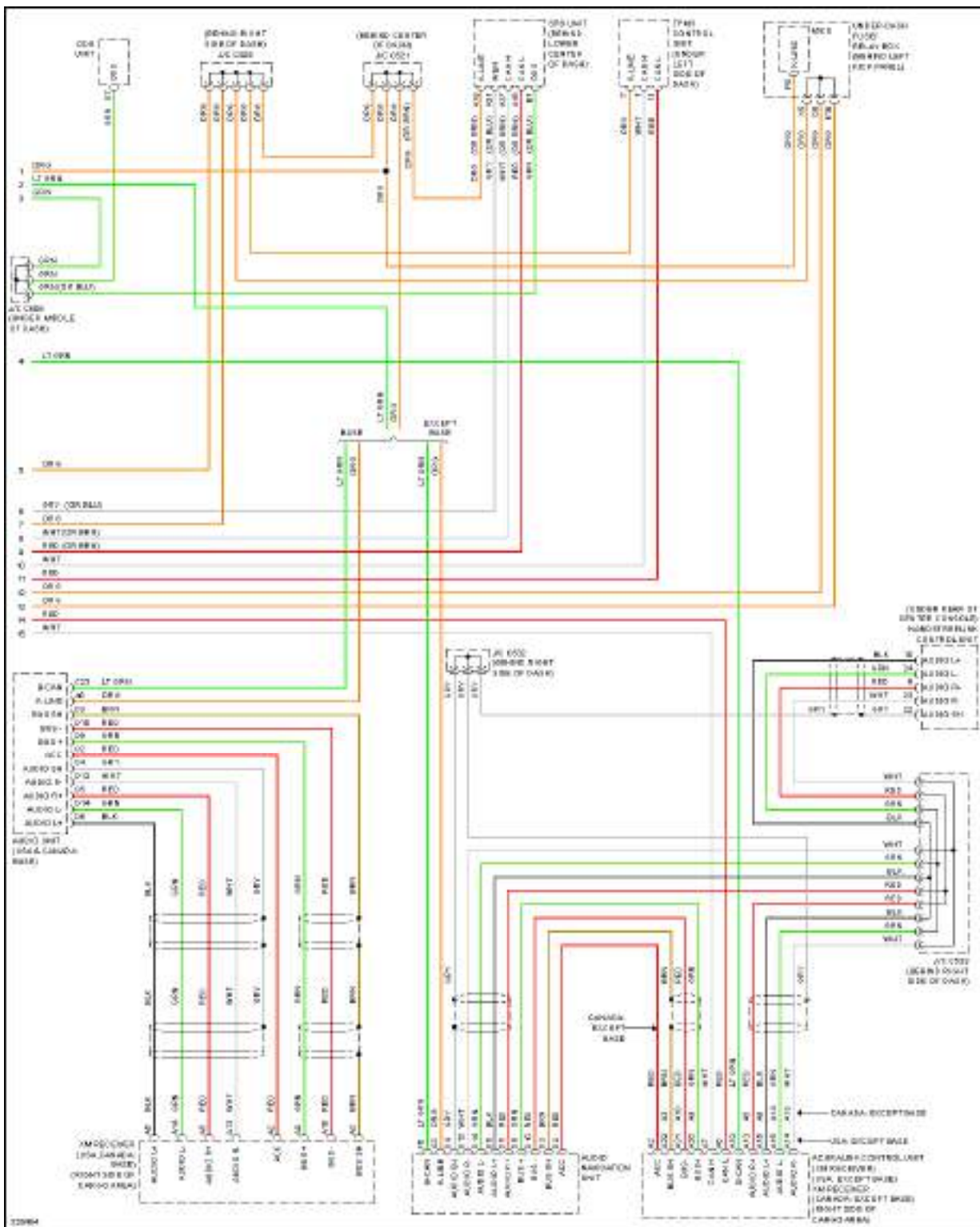
Fig. 10: Computer Data Lines Circuit (3 of 3)
